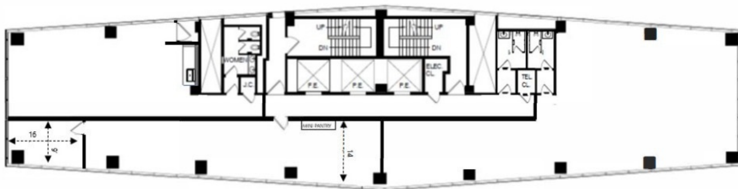
Suite 1820 1,499 SF
