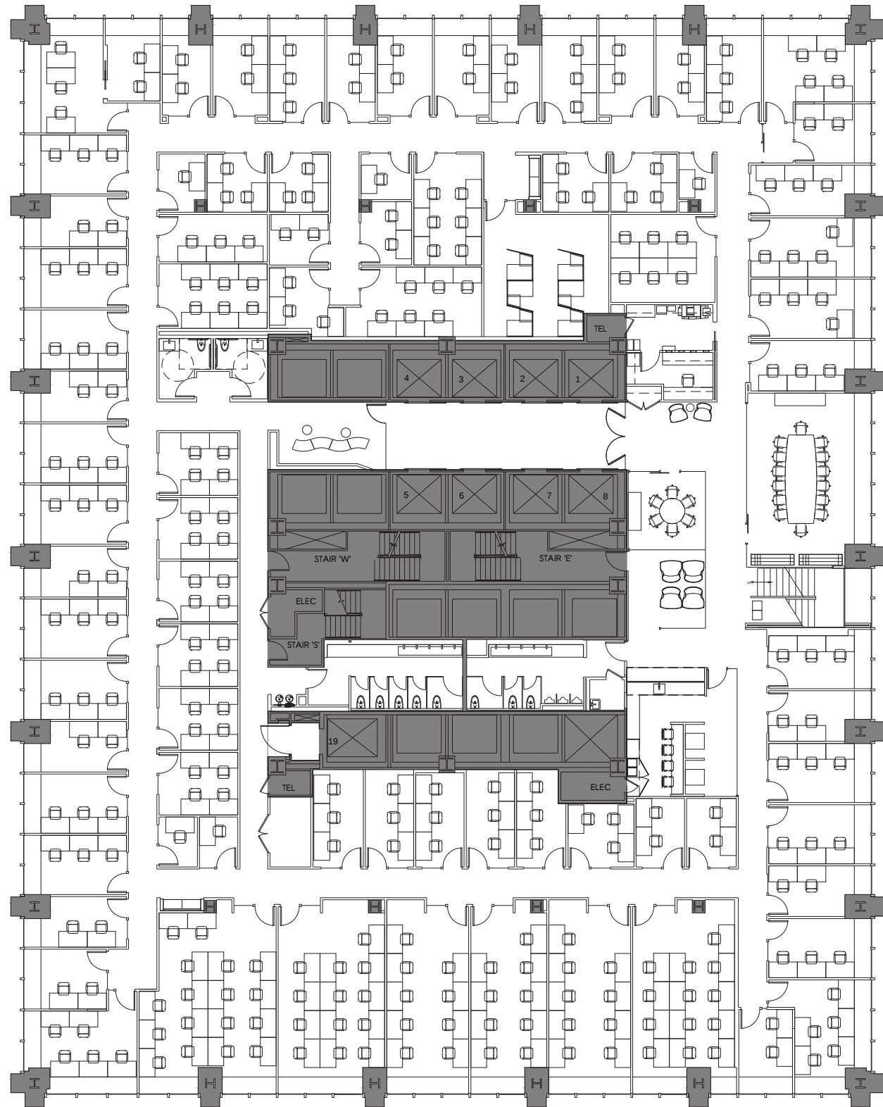
2ND FLOOR
