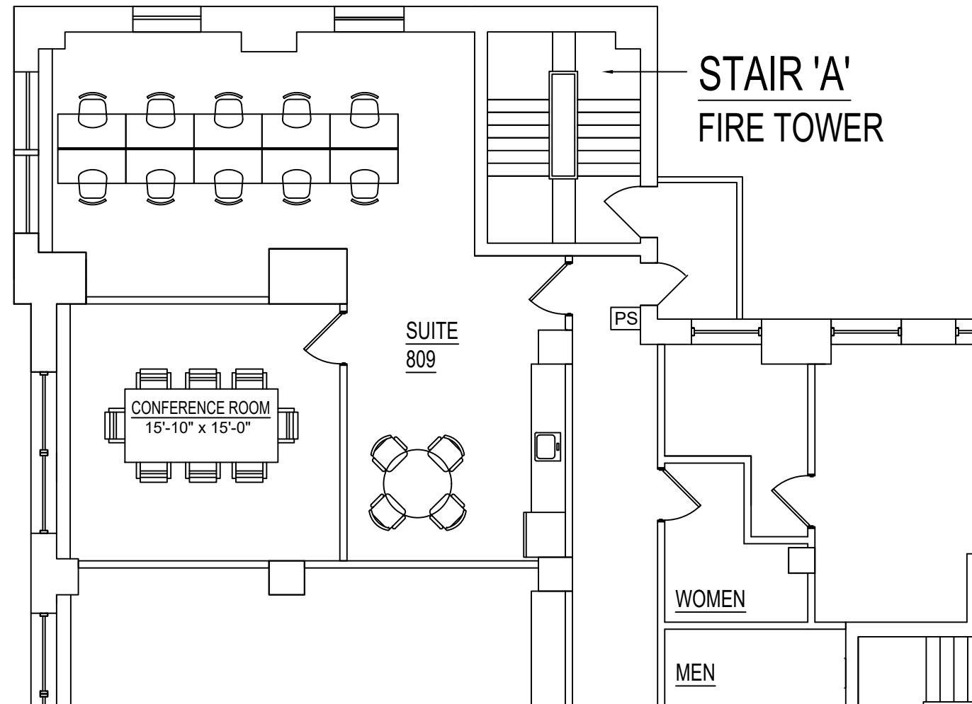
EIGHTH FLOOR PLAN - SUITE 809
