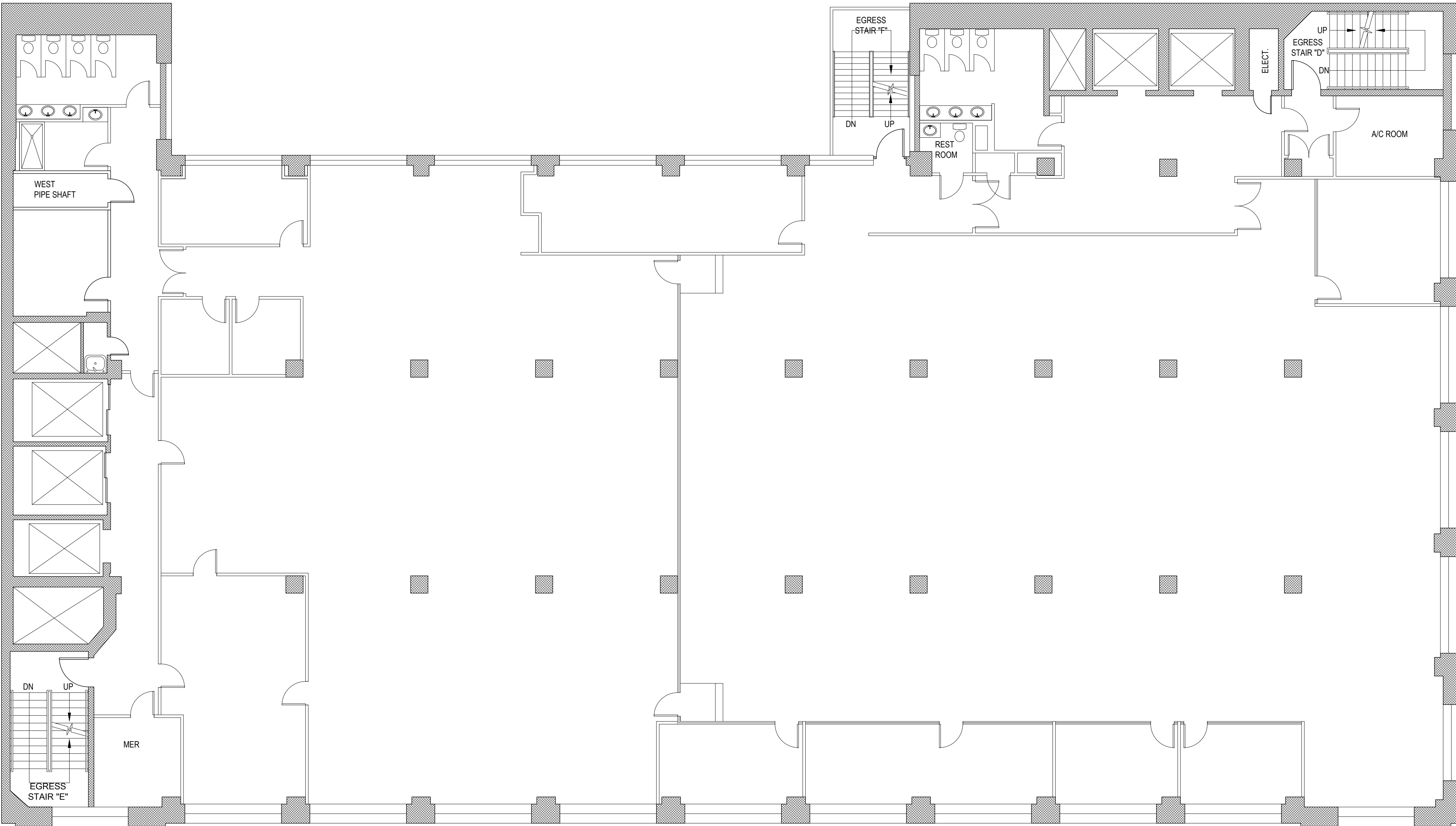
475 TENTH AVE - FOURTH FLOOR PLAN
