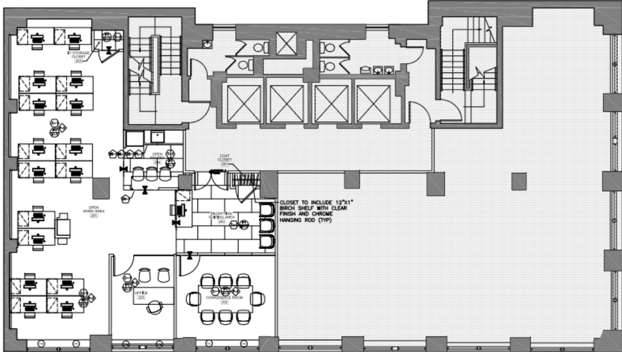
PARTIAL 2ND FLOOR FINISH PLAN (SCALE: 1/4" = 1'-0") 2
