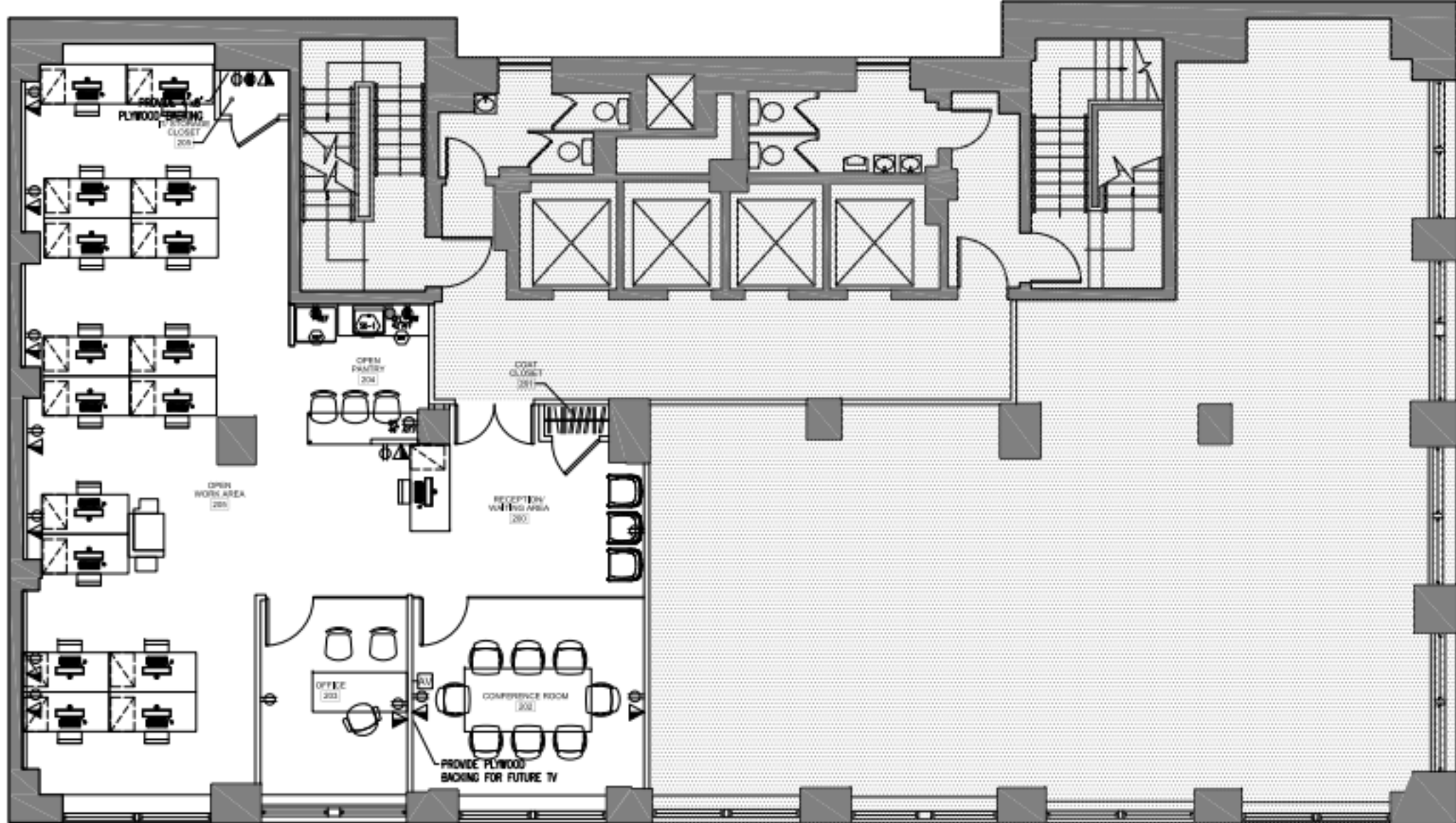
PARTIAL 2ND FLOOR POWER AND DATA PLAN (SCALE: 1/4" = 1'-0") 1
