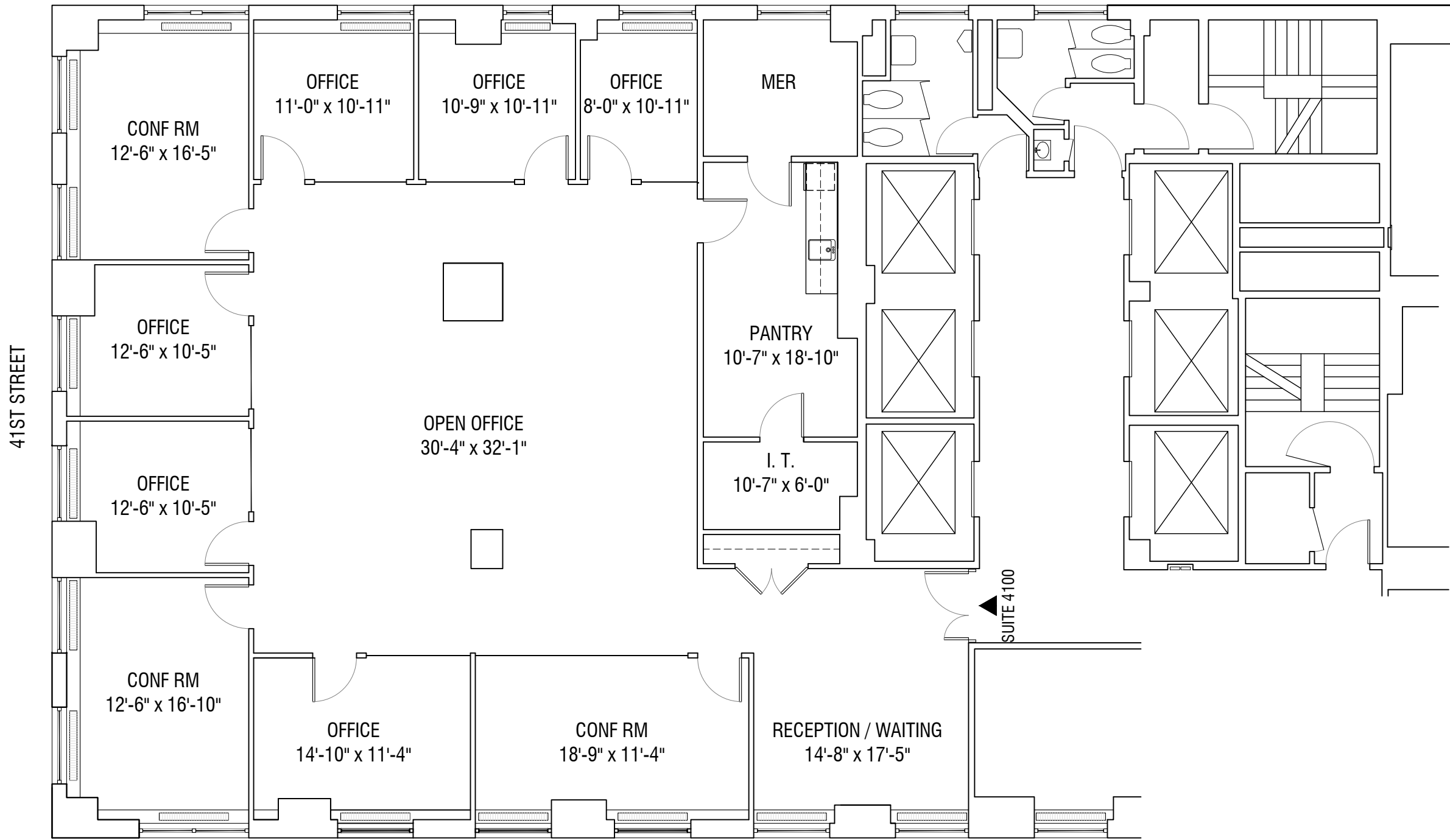
1 41ST FLOOR - PARTIAL FLOOR PLAN
