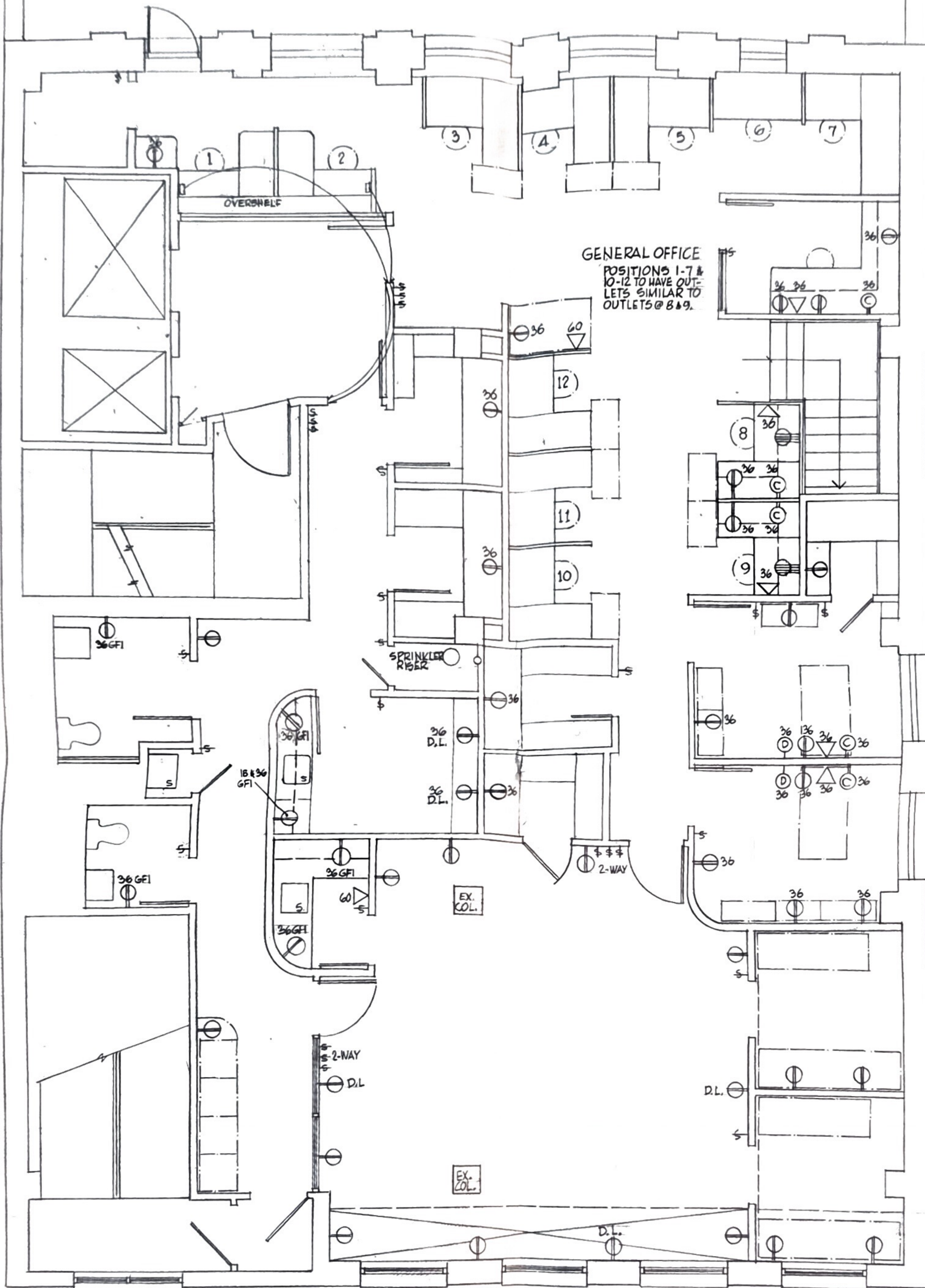
TENTH FLOOR POWER PLAN
