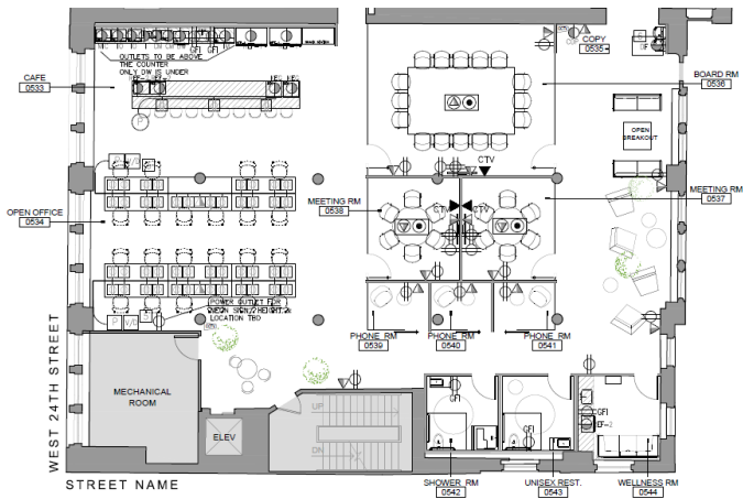
1 5th FLOOR ARCHITECTURAL POWER & VOICE/DATA PLAN SCALE: 1/8" = 1'-0"
