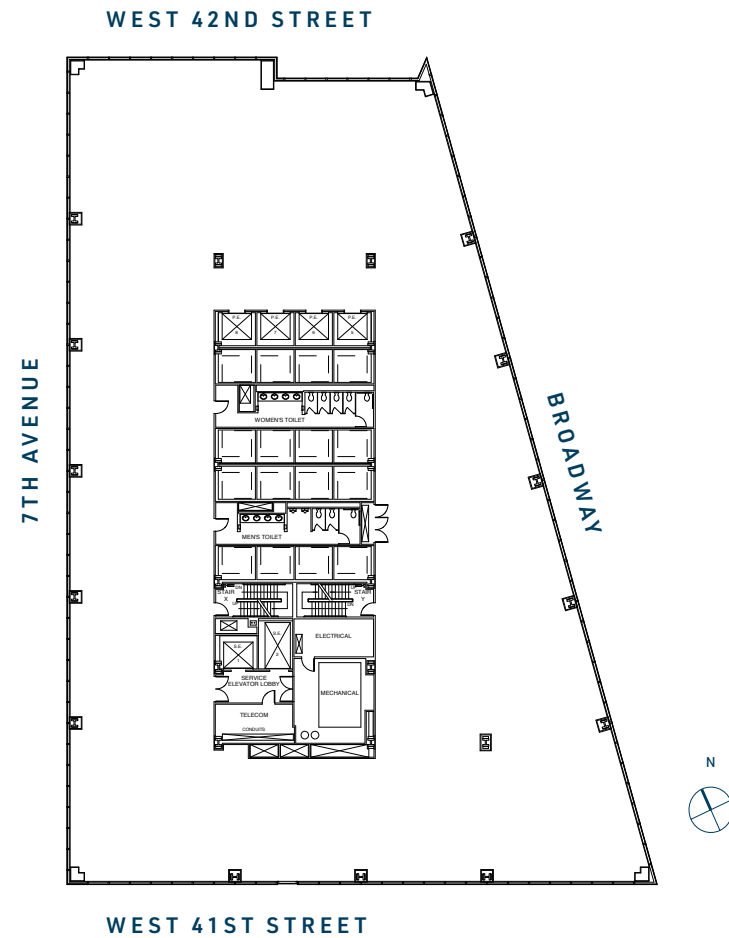
Core & Shell Plan 27,100 RSF
