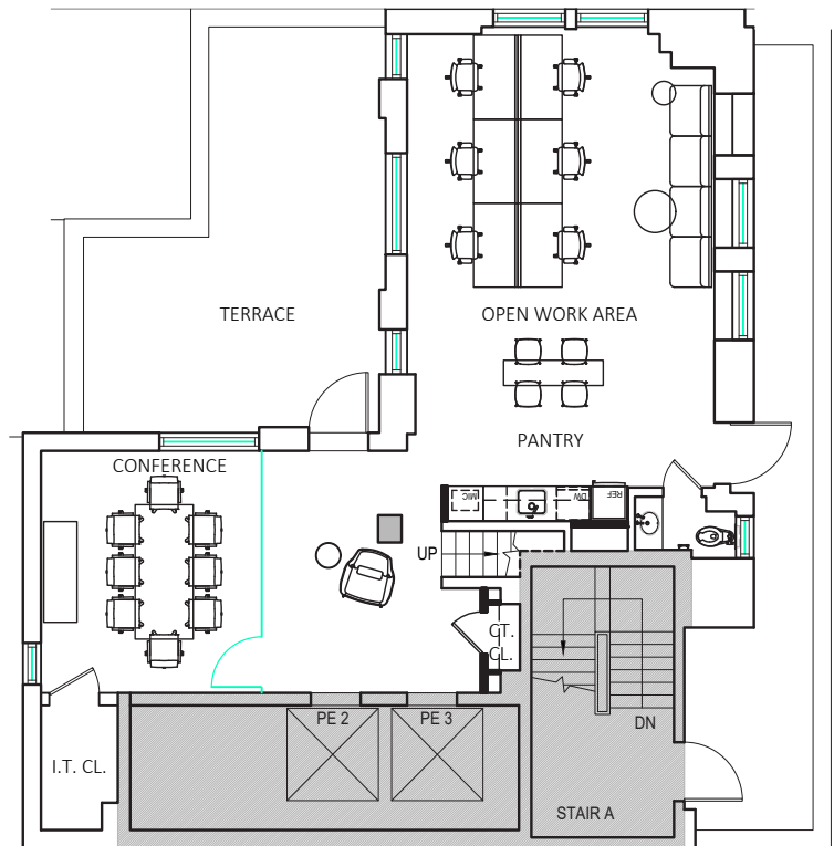
Penthouse Main
