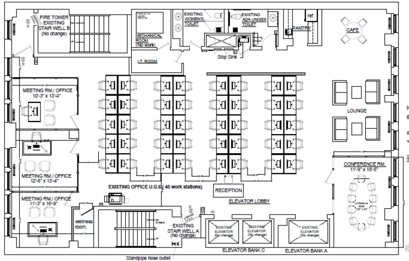
70 West 40th Street, 10th Fl. - Proposed Layout # 2 SCALE: 1/8"=10'
