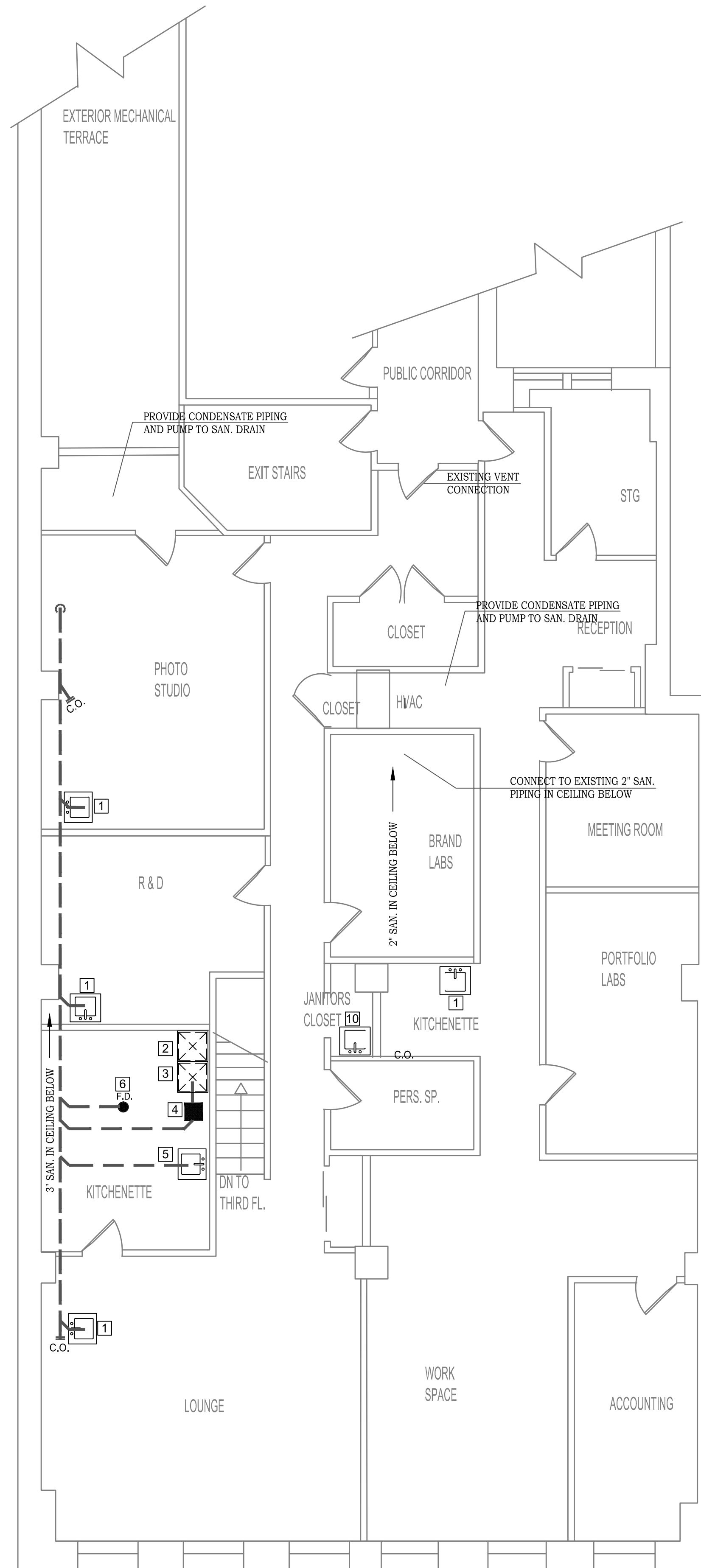
4TH FLOOR PLAN SC: 3/16"=1'-0"
