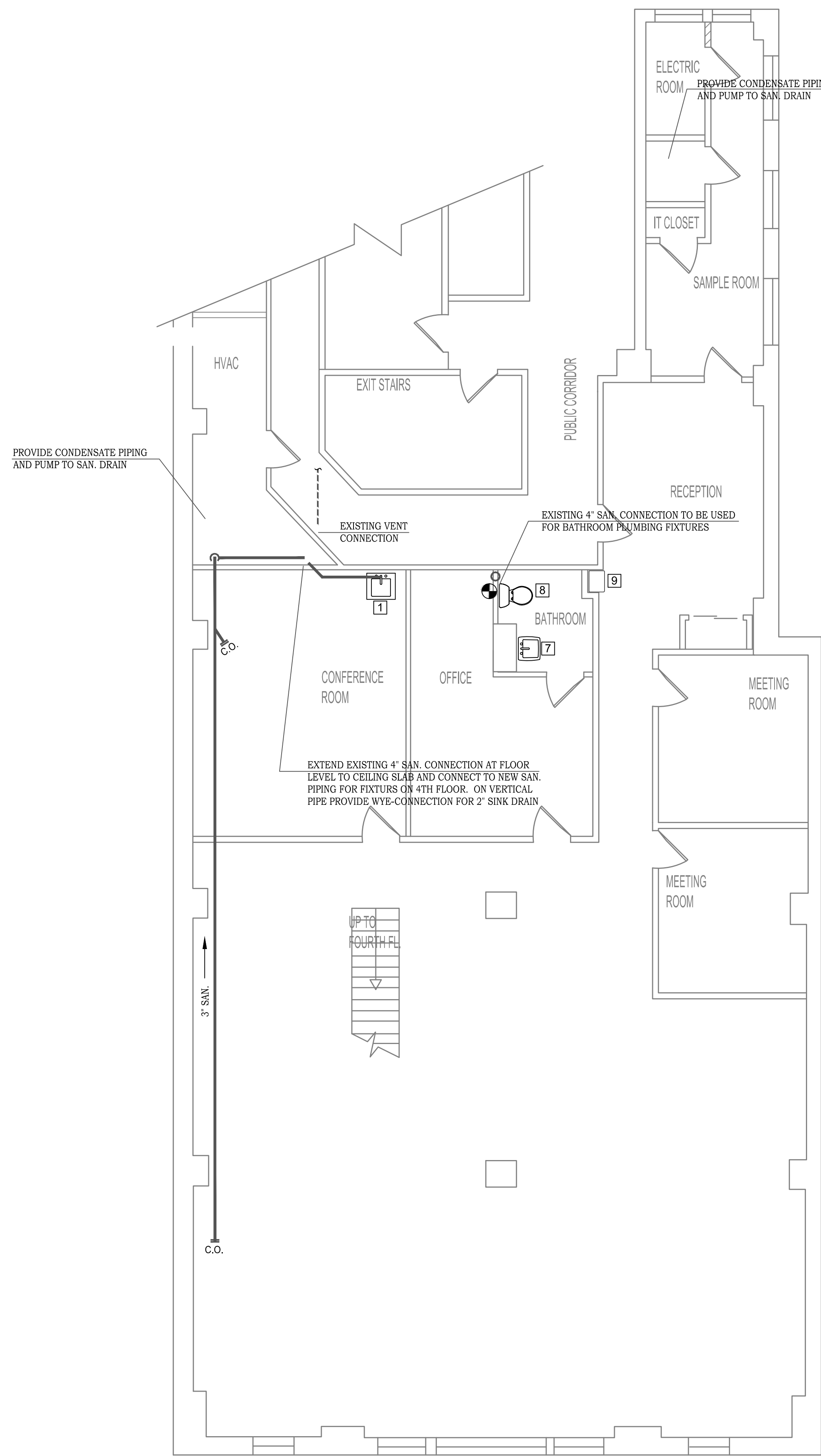
3RD FLOOR PLAN SC: 3/16"=1'-0"
