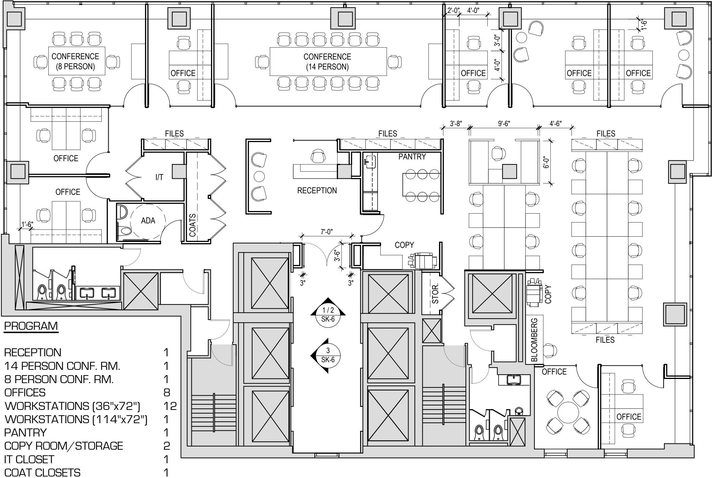
25TH FLOOR TEST FIT 9.15.2017 1/8"=1'-0"
