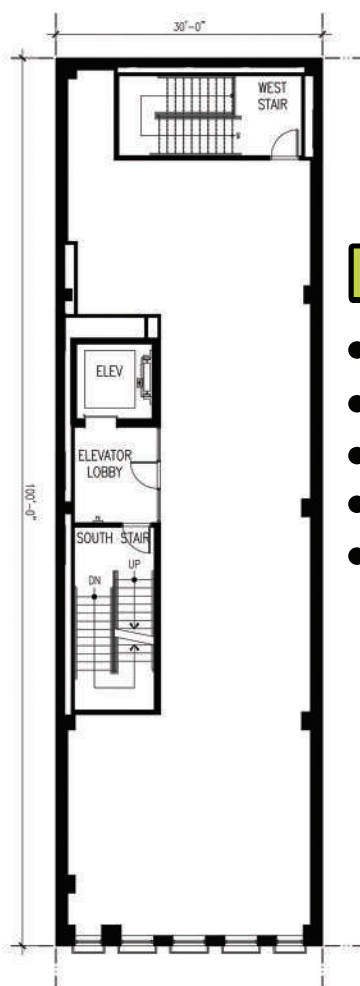
SIXTH FLOOR PLAN
