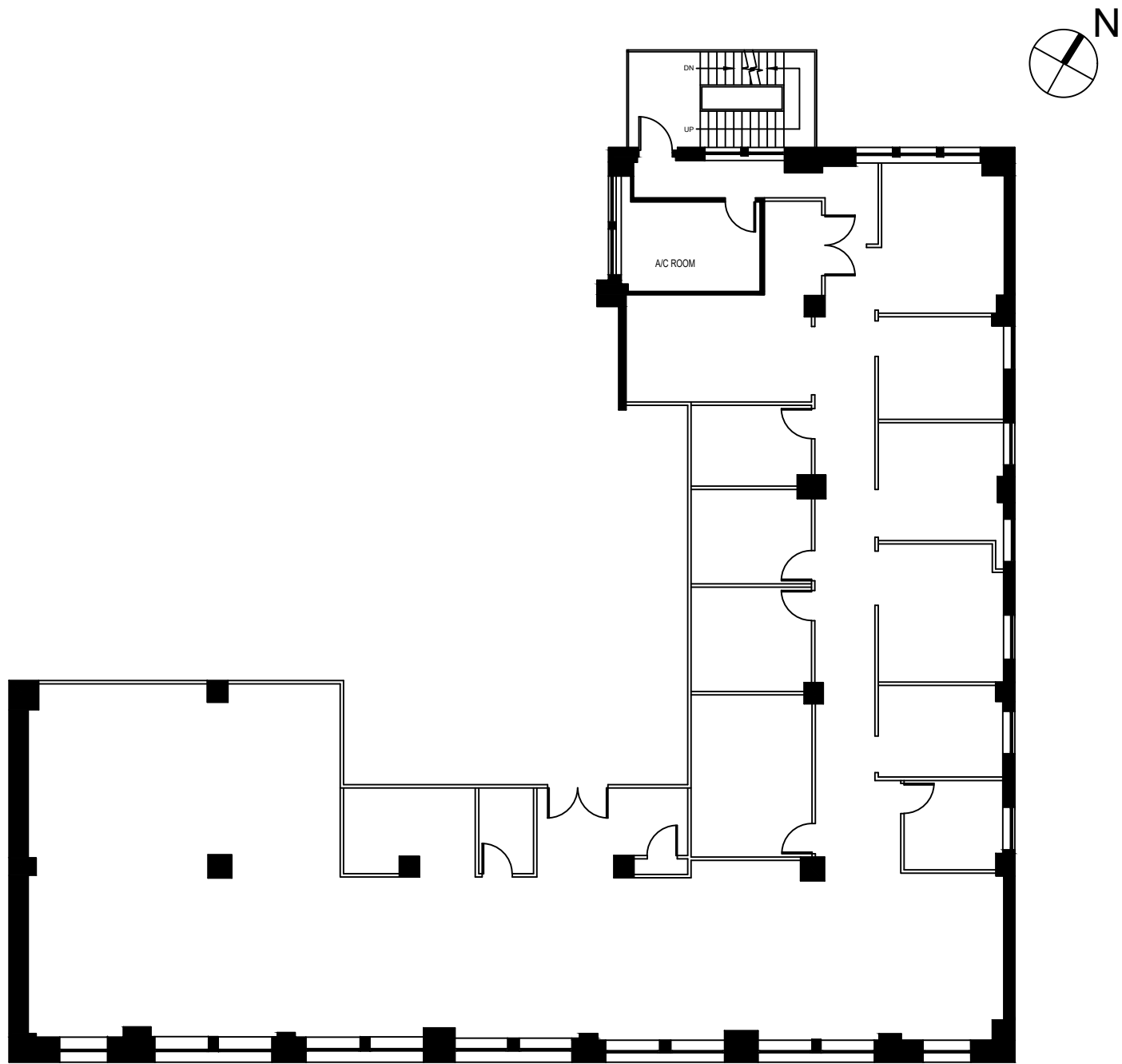
25 West 45th St. Suite 1001 - Existing Conditions 8,663 RSF
